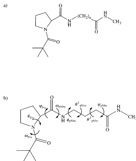
Scheme 1. a) Piv- 1 Pro-Xxx-NHMe, where Xxx = -\text{NH}-(\text{CH}_2)_n-\text{CO}- ( n=1 , Gly; n=2 , \beta -Gly; n=3 , \gamma -Abu; n=4 , \delta -Ava; n=5 , \epsilon -Acp). b) Definition of the backbone torsional angles in Piv- 1 Pro- \gamma -Abu-NHMe.
